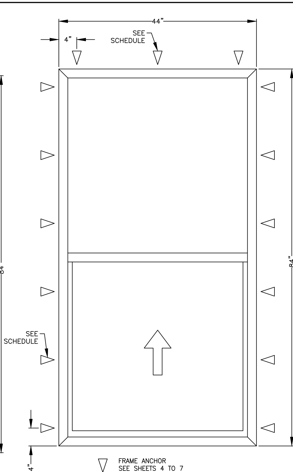
3540 SINGLE HUNG WINDOW (FINLESS AND FLANGE INSTALL) SIZE 44" X 84" DESIGN PRESSURE +/- 30 PSF
