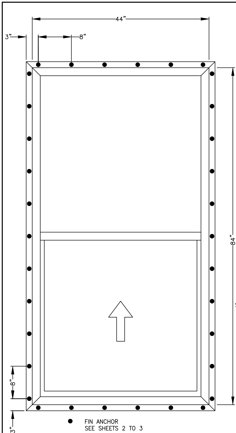
3540 SINGLE HUNG WINDOW (FIN INSTALL) SIZE 44" X 84" DESIGN PRESSURE +/- 30 PSF
